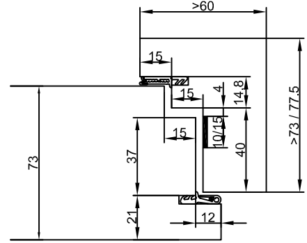
ClimaTop Eco MBW / LBW / PM / PL COMBIModul Blockrahmen / Cadre bloc
