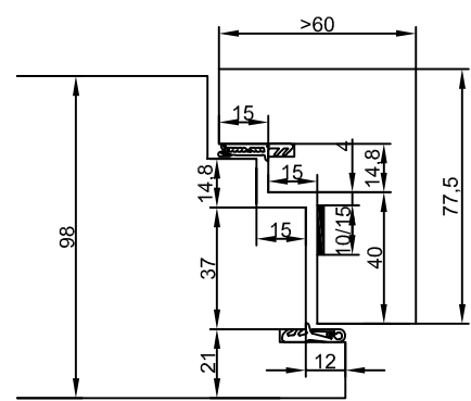
ClimaTop Plus MBW / LBW / PM / PL COMBIModul Blockrahmen / Cadre bloc
